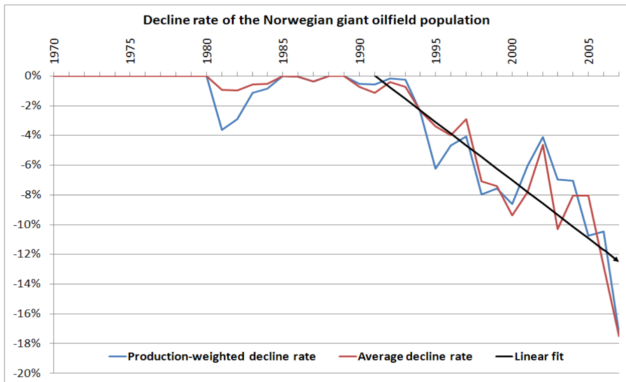
Figure 9: The decline of the Norwegian giant oilfields. Ultimately the onset of national decline could not be prevented and decline rates soared. Both the average and the production-weighted decline values agree well. Norway is an example of how technology can temporarily maintain production at the expense of a rapid future decline rate.
