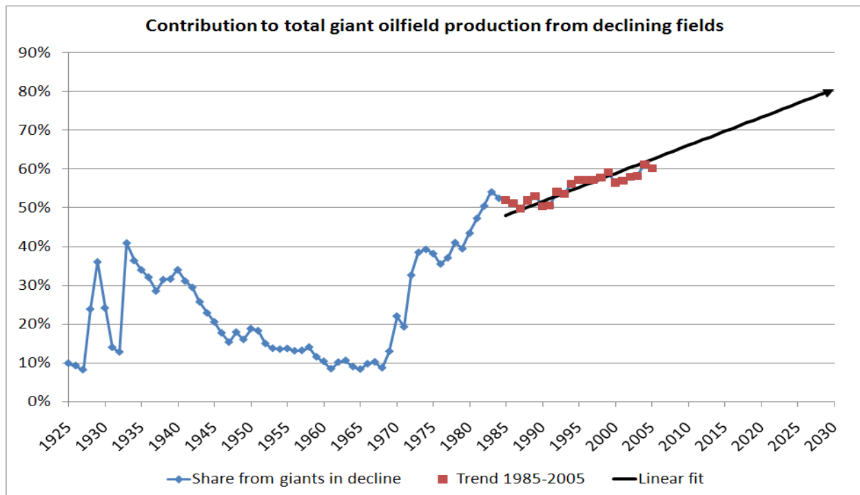
Figure 8: Contribution to total giant oilfield production from fields that have reached the onset of decline. In the 1920s oil was chiefly extracted in the US and when their giants started to decline, new giants fields all over the world were brought into production, which reduced the share from the declining fields. In the 1970s, production from many fields was interrupted for political reasons. Since 1985, the share from declining fields has been steadily increasing, despite the overall lack of political restrictions and turmoil. If extrapolated, this trend shows that over 80% of total giant oilfield production will come from fields in decline by 2030. However, the linear fit is only temporary and should be used with care if extrapolated far into the future.
