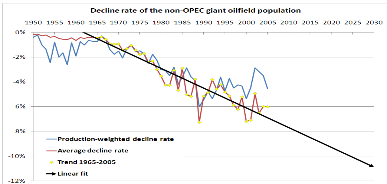
Figure 11: Decline rate of the non-OPEC giant fields. The average decline rate started to grow in 1965 and has been increasing as more and more giants reached the onset of decline. The deviation after 1995 was caused by the fall of the Soviet Union and the introduction of new technologies that managed to temporarily revive Russian giants.
